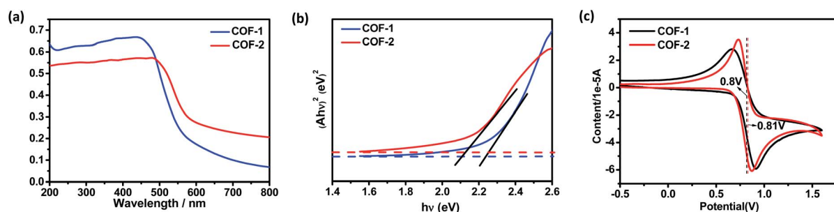
Fig. 5 (a) Solid-state UV spectra of the COFs. (b) Tauc plot for absorption spectra obtained with the Kubelka–Munk function and the linear fit for direct band gaps of the COFs. (c) Solid-state CV of the COFs with a scan rate of 50 \text{mV s}^{-1} .
