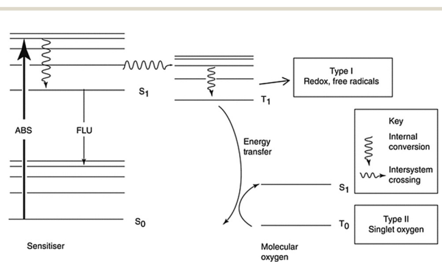
Fig. 1 The mechanism of photodynamic therapy. Reproduced with permission ref. 8.
