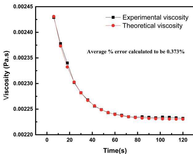
Fig. 11 Comparison between the experimental and theoretical values of the viscosities of 7-PSC at a constant shear rate.
