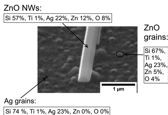
Fig. 8 SEM image of ZnO NWs grown on Ag (45 °C tilted) at a precursor concentration of 5 mM and growth time of 18 hours. EDX data (elemental percentage) have been shown at the points of ZnO NWs, ZnO grains, and Ag grains. The electron beam penetration depth is \sim 1 \mu\text{m} ; carbon and other contaminants have been ignored.
