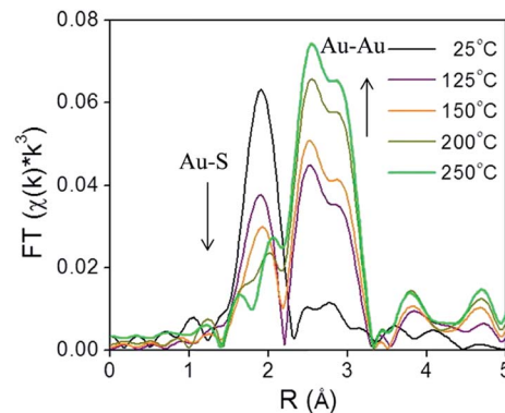
Fig. 4 Au L_3 edge EXAFS spectra in the R space of \text{Au}_{25}(\text{SR})_{18} clusters on carbon (with no phase shift correction). Reprinted with permission from ref. 54. Copyright 2013, American Chemical Society.
