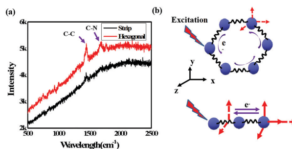
Fig. 8 (a) Raman spectra of different shaped \text{CH}_3\text{NH}_3\text{PbI}_3 perovskites and (b) schematic illustration of the Raman scattering for different shaped \text{CH}_3\text{NH}_3\text{PbI}_3 perovskites.
