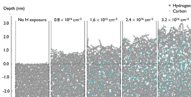
Fig. 8 Cross-sectional images of the a-C layer modified by H ions at different ion fluences.
