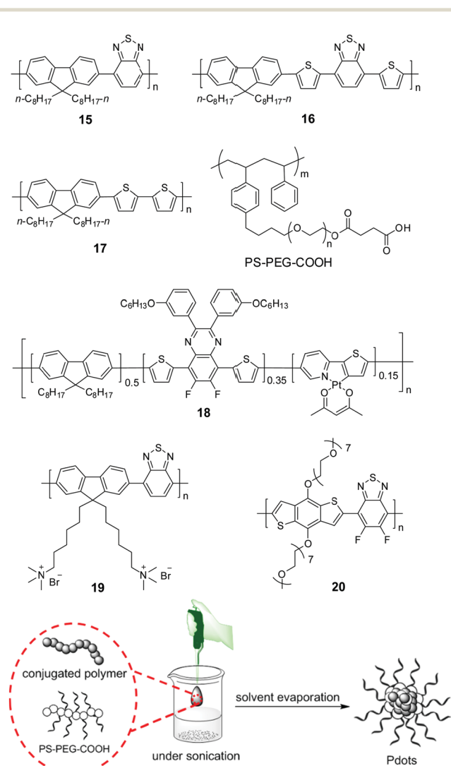
Fig. 6 Chemical structures of polymers 15–20 and preparation of polymer dots (Pdots) by the nano-precipitation method for photocatalytic \text{H}_2 production. The scheme is adapted with permission from ref. 82, Copyright 2016 Wiley-VCH.
