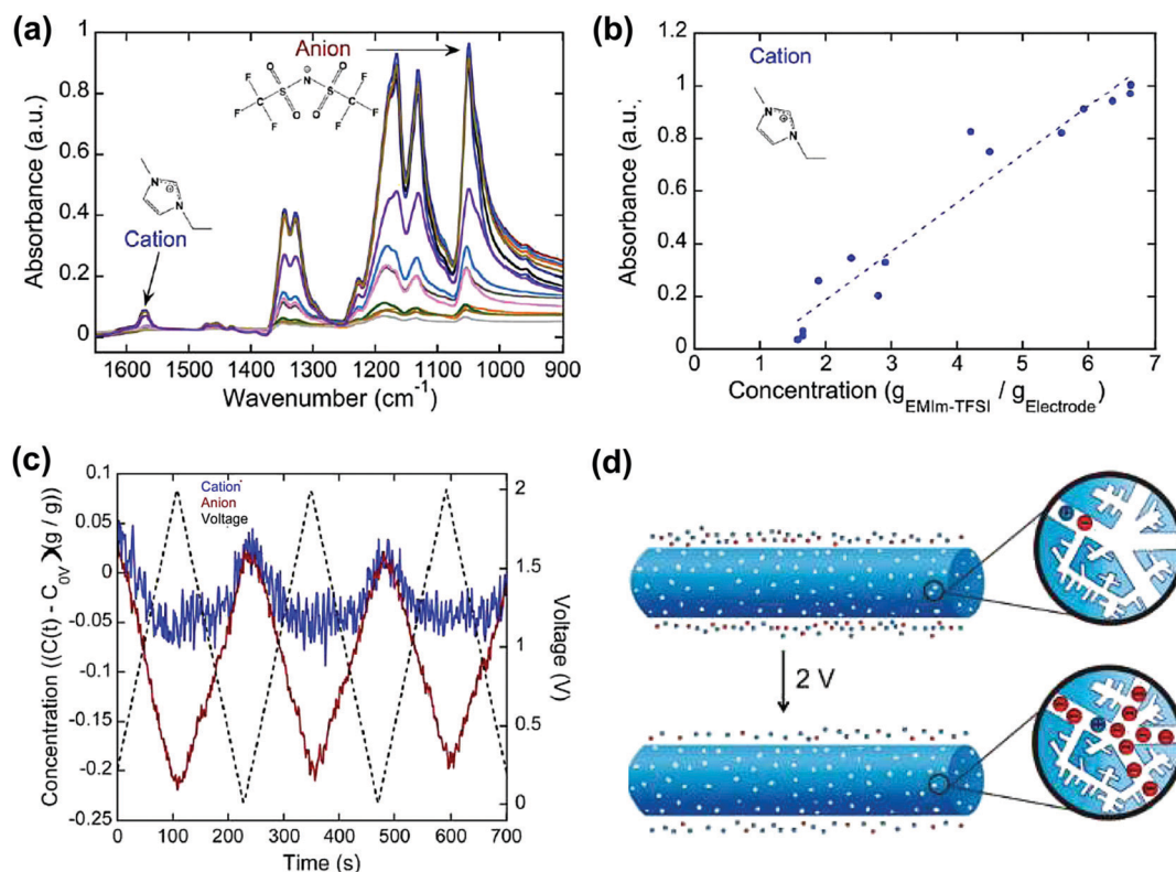
Fig. 13 (a) Infrared spectra of the NCNF electrodes with varying concentrations of the EMITFSI electrolyte ( 1.6 to 8.8 g EMITFSI g electrode −1 ). (b) Concentration–absorbance calibrations of the cation. The dotted lines represent linear regressions. (c) Operando infrared spectroelectrochemical results show the initialized time-resolved concentration (g EMI-TFSI g electrode −1 ) of EMI + cations and TFSI − anions in NCNFs from 0 to 2 V at 20 mV s −1 . (d) Illustration showing that a larger concentration of TFSI − anions than EMI + cations is in the nanopores of the positively charged NCNF nanopores. The figure is reproduced from ref. 228 with permission from American Chemical Society (copyright 2008).
