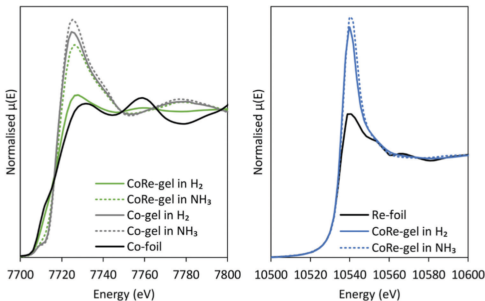
Fig. 9 XANES-spectra before and after switching from \text{H}_2 to \text{NH}_3 from the Co K-edge (left) and Re \text{L}_{\text{III}} -edge (right).
