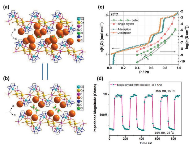
Fig. 17 (a and b) Packing diagrams of structures [\text{CaCo}(\text{notpH}_2)(\text{H}_2\text{O})_2](\text{ClO}_4) \cdot 4\text{H}_2\text{O} ( 28 ) (a) and [\text{CaCo}(\text{notpH}_2)(\text{H}_2\text{O})_2](\text{ClO}_4) \cdot 2\text{H}_2\text{O} ( 29 ) (b). (c) Proton conductivity and adsorption isotherms of 28 . (d) Impedance response and recovery time to RH variation between 55% and 95% for a single crystal of 28 along the [010] direction. Reprinted with permission from ref. 33. Copyright 2015, American Chemical Society.
