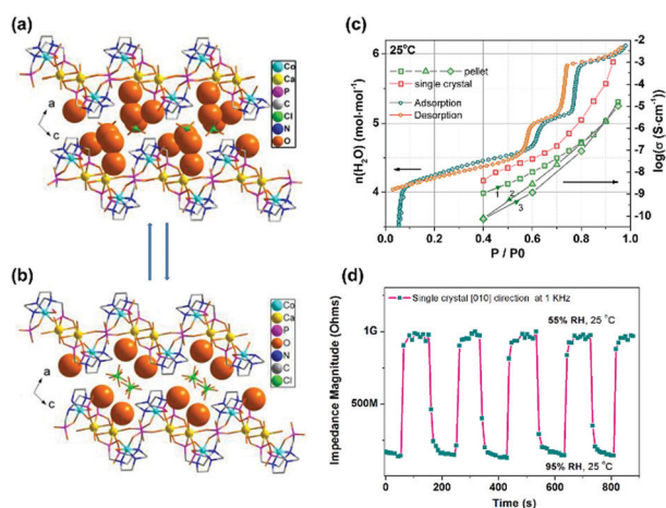
Fig. 17 (a and b) Packing diagrams of structures [\text{CoCa}(\text{notpH}_2)(\text{H}_2\text{O})_2](\text{ClO}_4)_4 \cdot 4\text{H}_2\text{O} ( 28 ) (a) and [\text{CoCa}(\text{notpH}_2)(\text{H}_2\text{O})_2](\text{ClO}_4)_2 \cdot 2\text{H}_2\text{O} ( 29 ) (b). (c) Proton conductivity and adsorption isotherms of 28 . (d) Impedance response and recovery time to RH variation between 55% and 95% for a single crystal of 28 along the [010] direction. Reprinted with permission from ref. 33. Copyright 2015, American Chemical Society.
