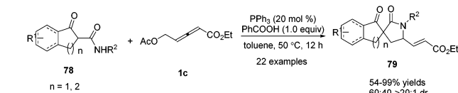
Scheme 25 \text{PPh}_3 -Catalysed (3+2) spiroannulation of \alpha -substituted secondary \beta -ketoamides with \delta -acetoxy allenates.
