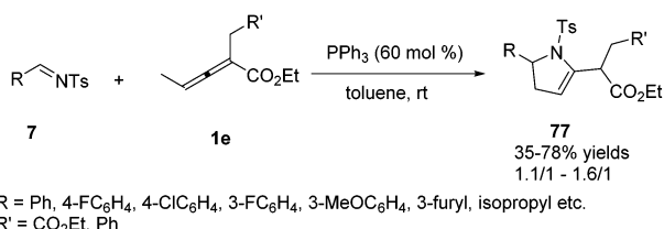
Scheme 24 \text{PPh}_3 -Mediated (3+2) cycloaddition reaction between bis-substituted allenates and N -tosylaldimines.
