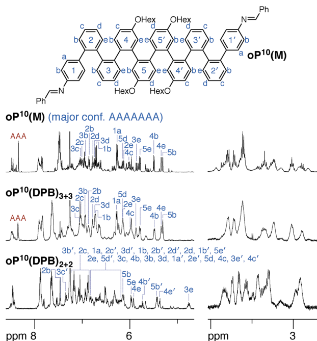
Fig. 8 ^1\text{H} NMR spectra (500 MHz, 0 °C) of \text{oP}^{10}(\text{M}) , \text{oP}^{10}(\text{DPB})_{2+2} , and \text{oP}^{10}(\text{DPB})_{3+3} . ^1\text{H} assignments for the major conformers are shown (blue). For \text{oP}^{10}(\text{DPB})_{2+2} , the assignments that are grouped together are listed in order from least- to most-shielded; chemical shifts for a minor conformation were also assigned (not shown).
