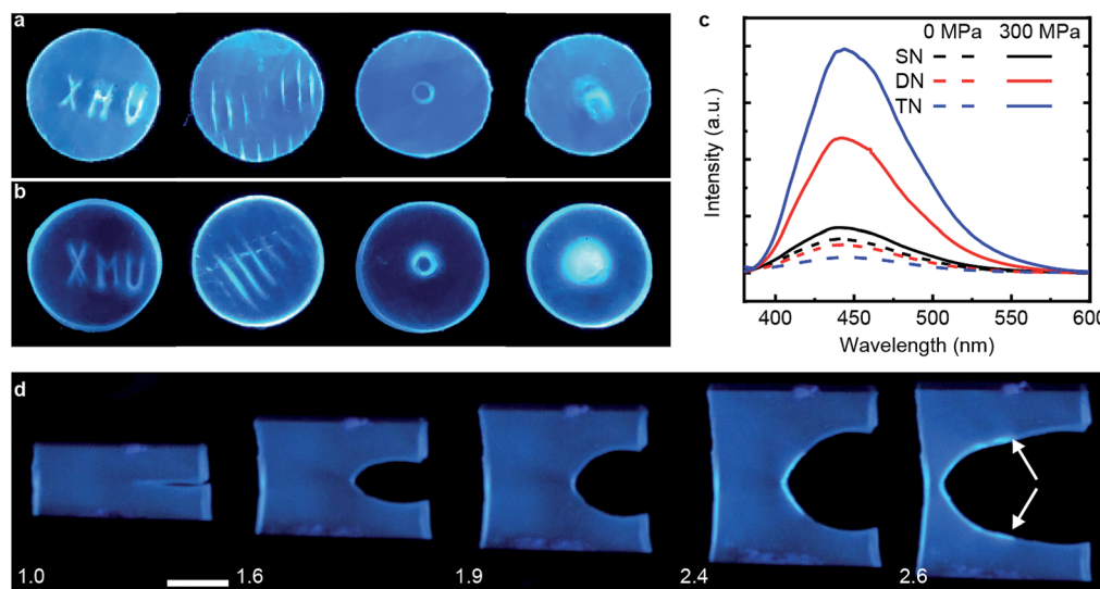
Fig. 2 Mechanochromic responses of DN and TN elastomers. (a and b) Spatial localized mechanochromism induced by compression on surfaces of DN (a) and TN (b) films. (c) Plot of fluorescent intensity under 365 nm UV excitation for uncompressed (dashed lines) and uniaxially compressed samples (300 MPa for 5 min, solid lines). (d) Fluorescent images (365 nm UV excitation) of a TN elastomer during crack propagation. Numbers are the stretch ratio along the vertical direction. The two white arrows indicate the start of the newly-formed surface. The scale bar is 1.0 cm.
