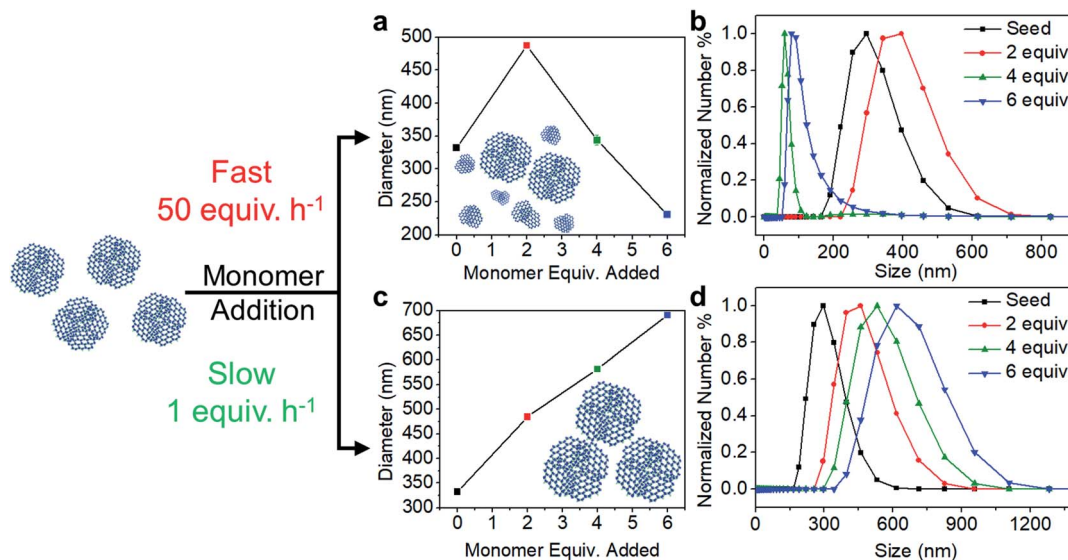
Fig. 3 Trend in the average size of particles with monomer addition at a fast rate of 50 equiv. h -1 and a slow rate of 1 equiv. h -1 . (a, c) Average size of particles with additional equivalents of monomers (b, d) corresponding number percent distribution.
