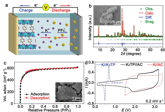
Fig. 1 (a) Schematic illustration of the KHC with the configuration K_2TP//DME\text{-based electrolyte}/AC ; (b) XRD pattern, Rietveld-refined profile, and SEM image (inset) of K_2TP ; (c) nitrogen sorption isotherm and SEM image (inset) of AC; and (d) CV curves of half batteries and the KHC.
