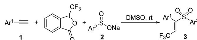
Scheme 2 Synthesis of ( E )- \beta -trifluoromethyl vinylsulfones.
