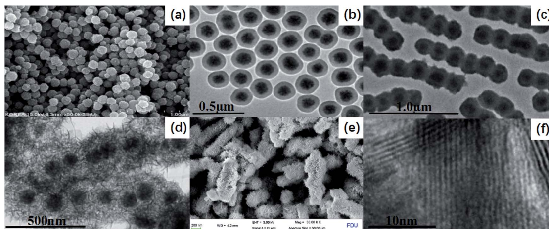
Fig. 2 SEM and TEM images: (a) SEM images of \text{Fe}_3\text{O}_4 nanoparticles, (b) TEM images of \text{Fe}_3\text{O}_4@\text{SiO}_2 nanospheres, (c) TEM image \text{Fe}_3\text{O}_4@\text{SiO}_2@\text{TiO}_2 , (d) TEM images of \text{PLYs-Fe}_3\text{O}_4@\text{TiO}_2 , (e) SEM image \text{PLYs-Fe}_3\text{O}_4@\text{TiO}_2 , (f) HRTEM image of the \text{TiO}_2 nanosheet.
