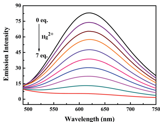
Fig. 4 Fluorescence titration spectra of luminogen 1 ( 2.0 \times 10^{-5} mol \text{L}^{-1} ) induced by \text{Hg}^{2+} (0–7.0 equiv.) in an acetonitrile solution. Excitation wavelength = 380 nm.
