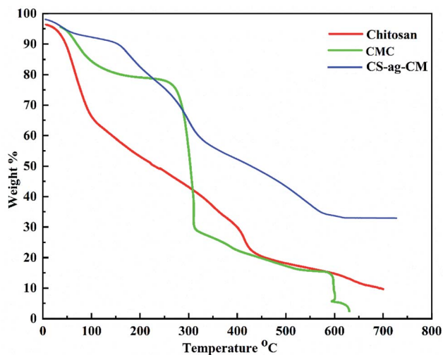
Fig. 4 TGA of CS, CM and CS-ag-CM.
