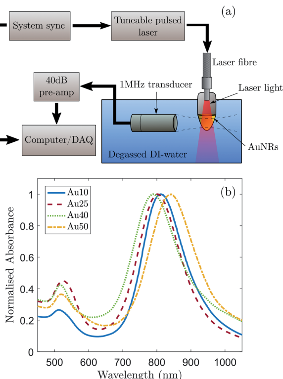
Fig. 1 (a) A schematic of the experimental setup used to detect the photoacoustic signals generated from AuNRs with longitudinal widths of 10, 25, 40 and 50 nm along with the (b) normalised measured absorbance spectra displaying SPR peaks at 811 \pm 2 nm, 803 \pm 2 nm, 790 \pm 2 nm, and 841 \pm 2 nm, respectively. The SPR of the Au50s showed a 50 nm shift compared with that of the Au40s, which can be ascribed to a combined effect of the AuNR width and aspect ratio on the SPR position of AuNRs.
