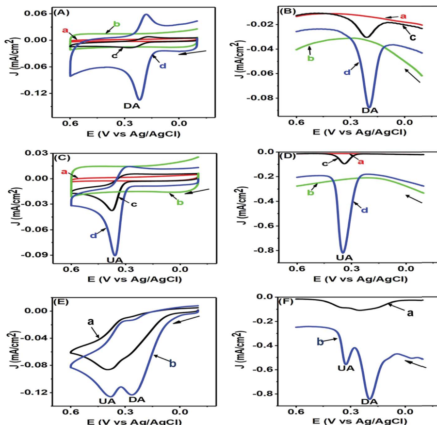
Fig. 7 CVs (A) and DPVs (B) of blank 0.1 M PBS solution of pH 7.0 (a and b) and 50 \mu\text{M} DA (c and d) in the same PBS of pH 7.0 at the GCE (a and c) and PTPCNs/GCE (b and d). CVs (C) and DPVs (D) of blank 0.1 M PBS of pH 7 (a and b) and 200 \mu\text{M} UA (c and d) in PBS of pH 7.0 at the GCE (a and c) and PTPCNs/GCE (b and d). CVs (E) and DPVs (F) of the mixture of 50 \mu\text{M} DA and 200 \mu\text{M} UA in 0.1 M PBS of pH 7.0 at the bare GCE (a) and PTPCNs/GCE (b).
