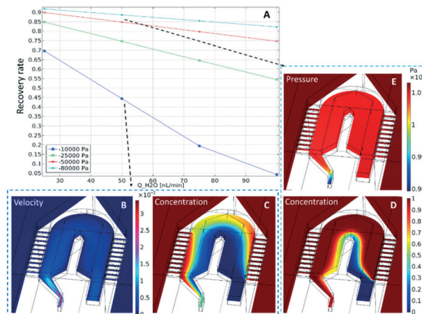
Fig. 2 COMSOL simulations to determine (A) the recovery rate of the \mu PPPS probe tip as a function of flow rate (x-axis) and outlet pressure (legend). Velocity profile ( m s^{-1} ) (B) and concentration profile (C) using 50 nL min^{-1} and -10 kPa outlet pressure. Pressure distribution (E) and concentration profile (D) for a flow rate of 50 nL min^{-1} and -80 kPa outlet pressure. Note that the pressure outside the probe is set to 1 bar (101.32 kPa).
