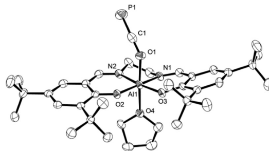
Fig. 3 Molecular structure of 2a-THF in the crystal 25 (ellipsoids are shown at 50% probability; hydrogen atoms and three toluene molecules are omitted for clarity). Selected bond distances [Å] and angles [°]: C1–P1 1.587(5), C1–O1 1.228(5), Al1–O1 1.920(3), Al1–O2 1.802(3), Al1–O3 1.796(2), Al1–O4 2.040(3), C1–O1–Al1 137.5(2), O1–C1–P1 178.5(3).
