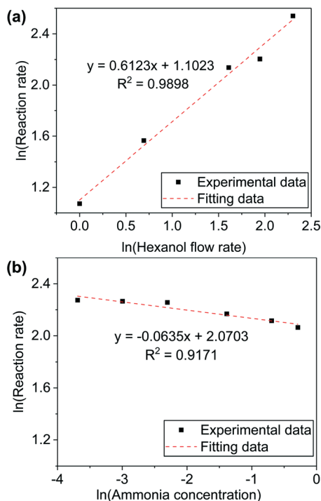
Fig. 2 Plots of ln(reaction rate) v.s. (a) ln(hexanol flow rate), hexanol flow rate was in unit of \mu\text{L min}^{-1} and flow rate of \text{NH}_3 and \text{N}_2 were 4 \text{mL min}^{-1} and 76 \text{mL min}^{-1} ; and (b) ln(ammonia concentration), flow rate of 1-hexanol was 5 \mu\text{L min}^{-1} and total gas flow rate was 80 \text{mL min}^{-1} by supplementing \text{N}_2 . Reaction rate was calculated as mmol of substrate converted per gram of catalyst per hour. 190 °C, 50 mg Ni/ \text{Al}_2\text{O}_3 -DP catalyst. GHSV = 1.28 \times 10^5 \text{ h}^{-1} .
