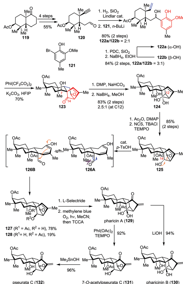
Scheme 22 Total synthesis of pharicin A, pharicin B, 7- O -acetylpsourata C and psourata C by Ding and co-workers.
