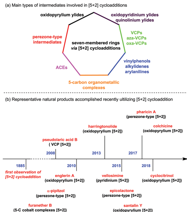
Fig. 1 (a) Main types of intermediates involved in [5+2] cycloadditions. (b) Representative natural products accomplished recently utilizing [5+2] cycloaddition as a key step.
