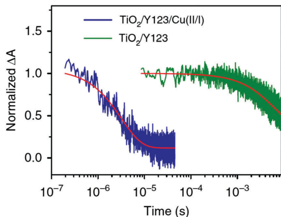
Fig. 9 Transient absorption spectra of Y123 -sensitized photoanodes inert (green) and in contact with the solid \text{Cu}^{\text{II/I}}(\text{tmb})_2 hole transport material. Reproduced from ref. 87 with permission from the Nature publishing group.
