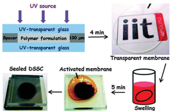
Fig. 21 Preparation of quasi-solid polymer electrolytes by swelling techniques. Reproduced from ref. 227 with permission from the Royal Society of Chemistry.
