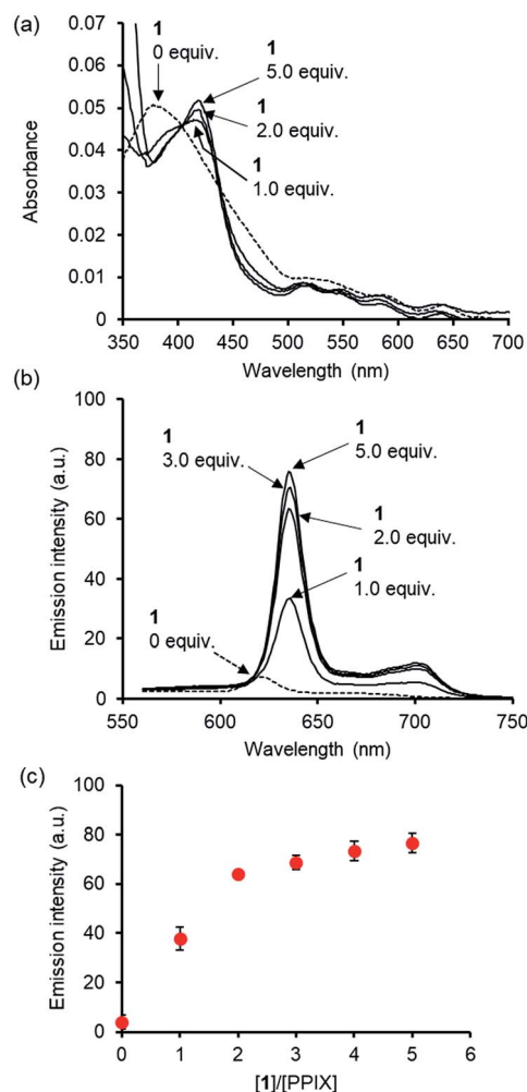
Fig. 7 (a) Typical UV-Vis spectra and (b) typical fluorescence emission spectra (excitation at 545 nm) of PPIX (1.0 \mu\text{M} ) in the absence and presence of 1 in DMSO/DMEM = 1 : 99 (v/v) at 25 ^{\circ}\text{C} . (c) Changes in mean emission intensity at 635 nm of PPIX in the presence of 1 . The data represent the mean \pm standard deviation of three independent experiments.
