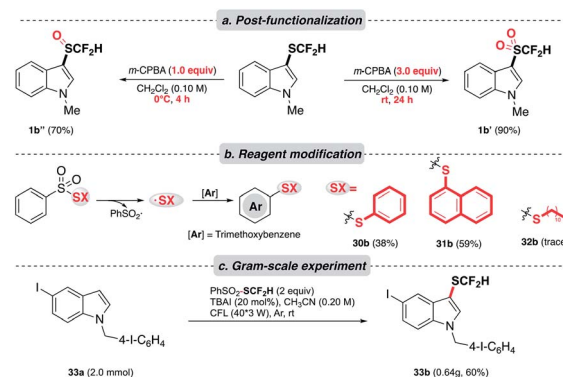
Scheme 4 Application. (a) Controlled oxidation of thioethers to corresponding sulfoxides and sulfones; (b) modified reagents to afford arythiolation products; (c) scaled-up experiments.
