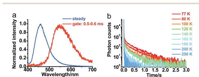
Fig. 4 (a) Normalized steady-state and time-gated emission spectra of the crystal of PXZT at room temperature in air. The energy of first excited singlet state E_S = 3.00 eV, the energy of first excited triplet state E_T = 2.55 eV, and the singlet-triplet splitting energy \Delta E_{ST} = 0.45 eV. (b) Transient photoluminescence decay spectra of the crystal of PXZT at different temperatures under Ar, \lambda_{\text{ex}} = 377 nm, \lambda_{\text{em}} = 560 nm.
