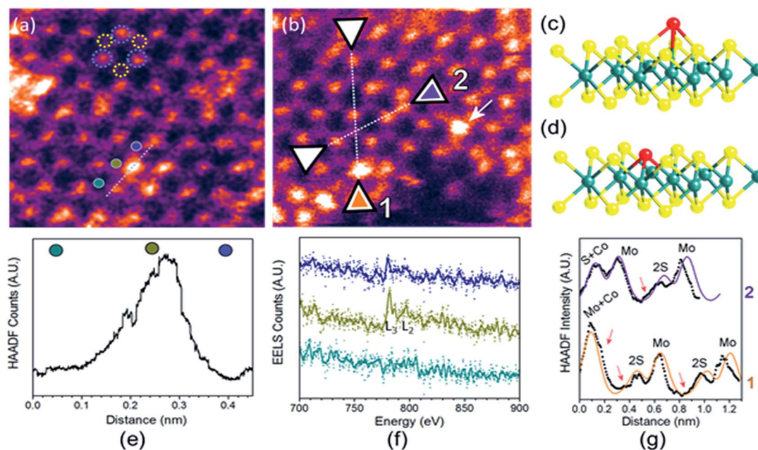
Fig. 3 (a) and (b) HAADF-STEM images of Co-SMo 2 . 29 Simultaneous acquisition of (c) Co at the Mo-atop site model and (d) Co at the S vacancy site model (e) ADF and (f) EELS acquired along the line in (a). (g) ADF intensity line profiles taken along the numbered lines 1 and 2 shown in (b) ( \langle 110 \rangle direction). The red arrows in the plot indicate sample drift during image acquisition.
