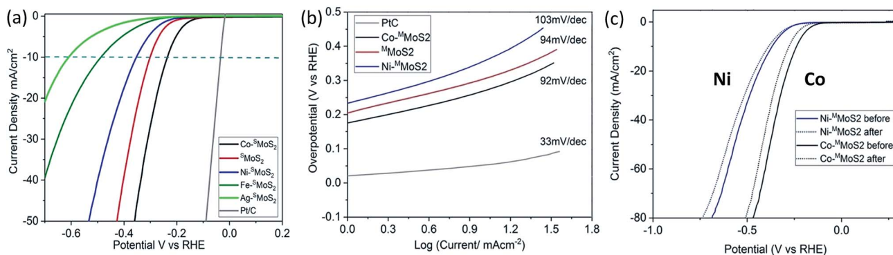
Fig. 2 HER activity analysis by linear sweep voltammetry, LSV. (a) LSV of the M-SMo 2 nanosheets and the reference 20% Pt/C in 0.5 M H 2 SO 4 at a scan rate of 2 mVs -1 . (b) Tafel plot of Co-SMo 2 , S-MoS 2 , Ni-SMo 2 and 20%Pt/C. (c) LSV of Co-SMo 2 and Ni-SMo 2 before and after 1000 repeat scans at a scan rate of 50 mV s -1 .
