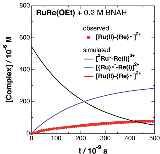
Fig. 4 Time profile of [\text{Ru(II)-(Re)}\cdot\text{-}]^{2+} (●) in the TRIR measurement of \text{RuRe(OEt)} in the presence of 0.2 M BNAH in an argon-saturated \text{CH}_3\text{CN/TEOA} (5:1 v/v) solution after 532 nm excitation. The kinetic simulation results for [\text{}^3\text{Ru}^*\text{-Re(I)}]^{3+} , [\{\text{Ru}\}\cdot\text{-Re(I)}]^{2+} , and [\text{Ru(II)-(Re)}\cdot\text{-}]^{2+} are also shown (solid lines).
