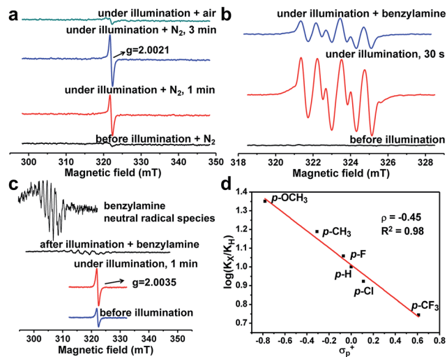
Fig. 1 (a) ESR detection of the electron transfer process in PCN-222. (b) ESR detection of \text{O}_2^{\cdot-} generation over PCN-222 trapped by DMPO. (c) The detection of hole-involved intermediates in PCN-222. (d) Hammett plot for the oxidation of benzylamine and its para -substituted derivatives photocatalyzed by PCN-222. All ESR tests were described in detail in the Experimental section.
