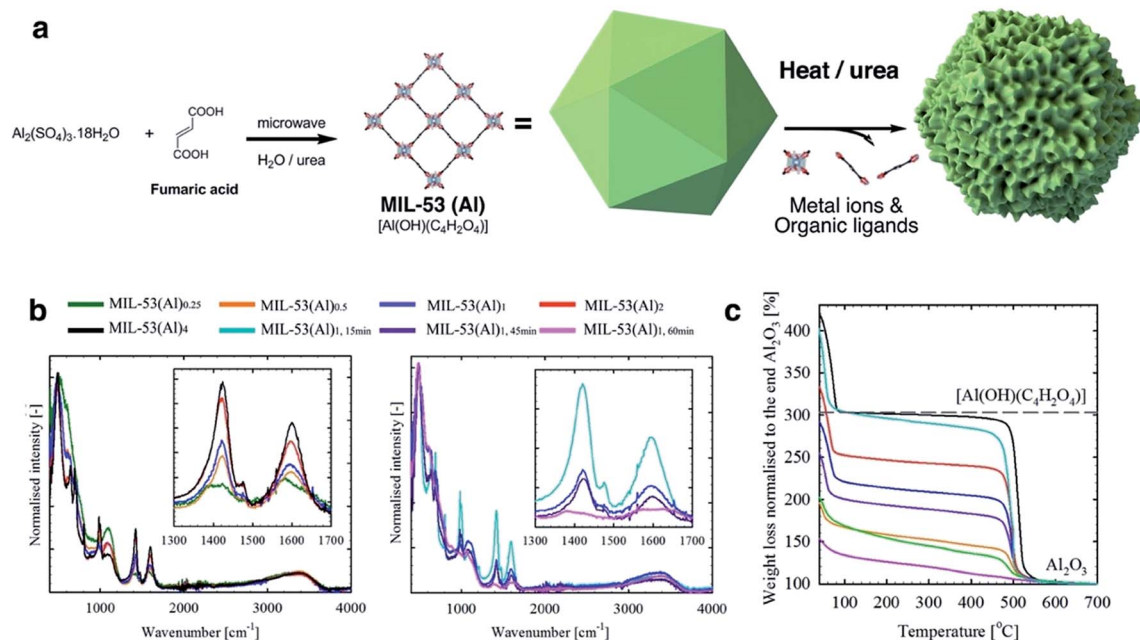
Fig. 1 (a) Schematic diagram of the MIL-53 synthesis and defect generation; (b) normalised ATR-FTIR spectrum for MIL-53(Al) samples (left: different stoichiometric ratios, and right: different reaction time). Insets show the characteristic signals (anti-symmetric \nu_{\text{asym}}(\text{C}=\text{O}) and symmetric \nu_{\text{sym}}(\text{C}=\text{O}) vibrations for carboxylate at ca. 1603 and 1426 cm -1 , 31 respectively) for the coordinating fumarate ligands; (c) normalized TGA curves for MIL-53(Al) samples. Black dashed-line indicates the theoretical weight for perfect MIL-53(Al) ([Al(OH)(C 4 H 2 O 4 )]) at 250 °C. The IR and TGA data are measured for the dried samples.
