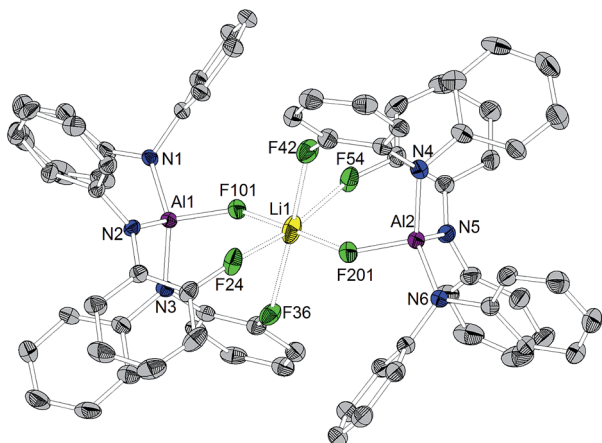
Chart 4 Molecular structure of [\text{CPh}_3]^+[\text{[(C}_6\text{F}_5)_2\text{N}]_3\text{AlF-Li-FAl(N(C}_6\text{F}_5)_2)_3}]^- (ellipsoids with 30% probability, non-coordinating fluorine atoms, the cation and two toluene molecules omitted for clarity). Selected bond lengths/Å and angles/°: Al1–N1 1.862(3), Al1–N2 1.859(4), Al1–N3 1.857(3), Al1–F101 1.714(3), Al2–N4 1.865(4), Al2–N5 1.859(4), Al2–N6 1.861(4), Al2–F201 1.710(3), Li1···F101 1.793(9), Li1···F201 1.809(9), Li1···F24 2.185(12), Li1···F36 2.392(10), Li1···F42 2.280(10), Li1···F54 2.287(12), N1–Al1–N2 113.51(15), N2–Al1–N3 102.24(16), N1–Al1–N3 123.30(16), N1–Al1–F101 99.83(15), N2–Al1–F101 114.48(15), N3–Al1–F101 103.57(14), N4–Al2–N5 102.41(17), N5–Al2–N6 115.61(17), N4–Al2–N6 122.56(17), N4–Al2–F201 102.66(15), N5–Al2–F201 112.48(16), N6–Al2–F201 100.55(16).
