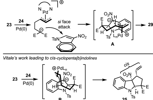
Scheme 8 Hyland's diastereoselective synthesis of cyclopenta[b]indolines.
