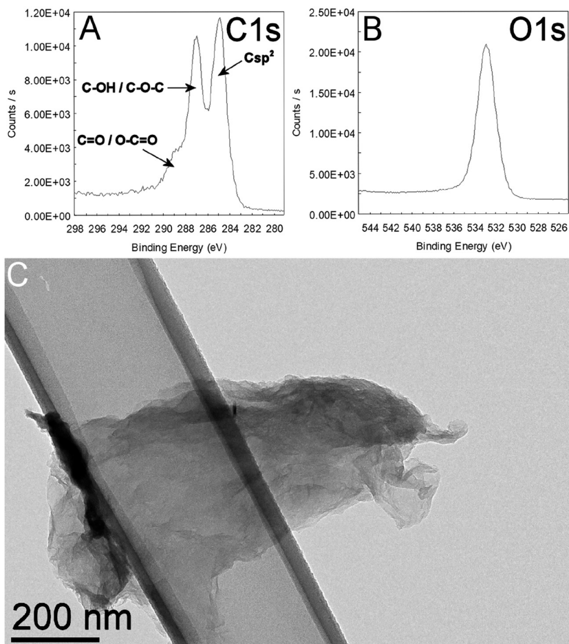
Fig. 1 XPS analysis of GO showing details of the C1s (A) and O1s (B) bands. A typical TEM image of the GO material is shown in (C).
