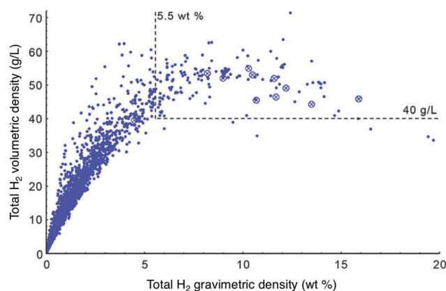
Fig. 2 Theoretical total volumetric vs. gravimetric capacities for various materials at 77 K and 35 bar, compared with the DOE 2025 system targets ( 5.5 \text{ wt}\% and 40 \text{ g L}^{-1} , as outlined by dashed lines). Adapted with permission from J. Goldsmith, A. G. Wong-Foy, M. J. Cafarella and D. J. Siegel, Chem. Mater. , 2013, 25 , 3373. Copyright 2008 American Chemical Society.
