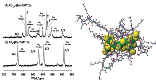
Fig. 6 ^{113}\text{Cd} -NMR spectra recorded for (A) \text{Cd}_{7/11}\beta -rhMT 1a showing the presence of 7 unique sites and (B) \text{Cd}_8 -rhMT 1a showing the presence of only 4 sites with unique chemical shifts. (C) A proposed structure for the \text{Cd}_8 -rhMT 1a using a molecular model. Reproduced from ref. 48 with the permission of the American Chemical Society.
