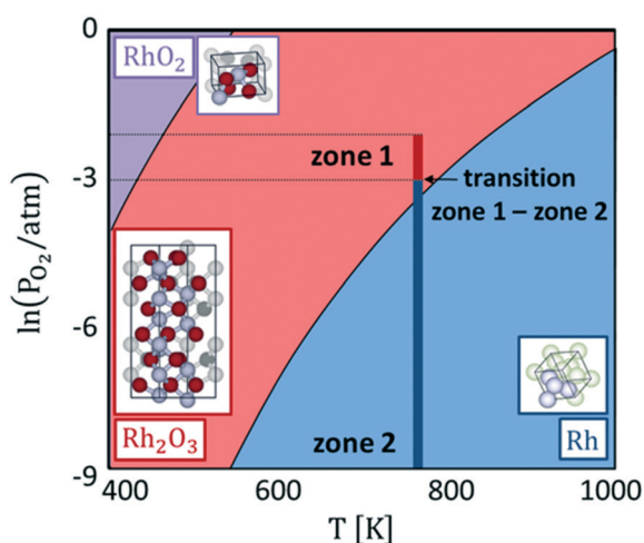
Fig. 2 Bulk phase diagram of Rh (in blue), corundum Rh 2 O 3 (in red) and rutile RhO 2 (in purple). In dark red and dark blue are the ranges of conditions that characterize the first and the second zone of the CPO reactor at 773 K and 1 atm.
