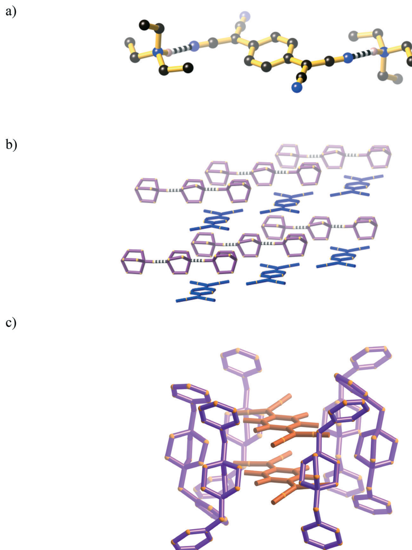
Fig. 18 a) Two \text{HNEt}_3^+ cations H-bonding to a \text{TCNQ}^{2-} anion in (\text{HNEt}_3)_2\text{TCNQ} (93). b) A view of [(\text{dabco-H}^+)_2(\text{dabco})]\text{TCNQ} (95). The internally H-bonded \text{dabcoH}^+-\text{dabco-H}^+\text{dabco} trimers (purple) interact electrostatically with strips of \text{TCNQ}^{2-} anions (blue). c) The structure of \text{dbdab-F}_4\text{TCNQ} (96) showing a pair of \text{F}_4\text{TCNQ}^{2-} units (orange) surrounded by \text{dbdab} cations (purple).
