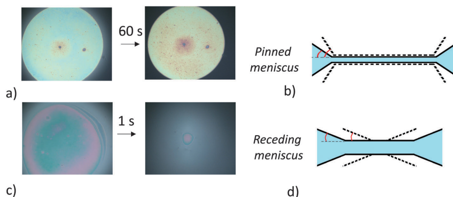
Fig. 4 Photographic images and schematic diagrams of thin liquid foams films during adhesion test for 1.5% mol BIS microgels. (a) and (b) 0.1% wt sample. (c) and (d) 1% wt sample.
