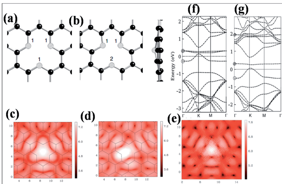
Fig. 28 (a) Top view of a fully relaxed non-reconstructed vacancy ( D_{3h} -symmetry of graphene). (b) Top and side views of the reconstructed vacancy with C_s -symmetry. (c–e) STM computed images for the single C-vacancy in graphene with a positive tip potential of 0.2 V. (c) D_{3h} vacancy; (d) C_s vacancy. (e) Average of the three equivalent C_s structures rotated by \pm 2\pi/3 . (f, g) Comparison of the DFT-LDA calculated band structures of graphene with mono-vacancies of different symmetries: (f) D_{3h} symmetry and (g) C_s symmetry. The shaded and empty circles respectively indicate the \sigma and \pi bands. The Fermi level is set to zero. Reproduced with permission. 309 © 2007 American Physical Society.
