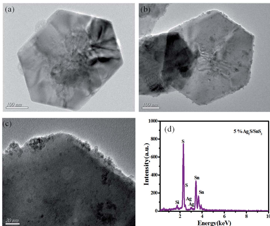
Fig. 2 TEM images of (a) SnS 2 ; (b and c) 1% Ag 2 S/SnS 2 composite; (d) EDS analysis of 5% Ag 2 S/SnS 2 composite sample.
