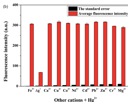
Fig. 2 (a) Fluorescence spectra of Z-3 and Z-3 + \text{Hg}^{2+} in the presence of 10 equiv. various metal ions in DMSO/ \text{H}_2\text{O} (v/v, 3 : 2; buffered with HEPES, pH = 7.20) solutions; (b) error bar of Z-3 + \text{Hg}^{2+} in the presence of various cations.
