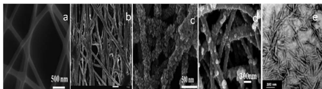
Fig. 1 SEM images of various types of CNF synthesized from cotton (a) natural electrospun CNF 56 (b) aligned CNF (scale bar 1 μm) 54 (c): CdS functionalized CNF 33 (d): CeO 2 functionalized CNF 56 (e): CNF prepared by acid hydrolysis 52 (adopted with permission).
