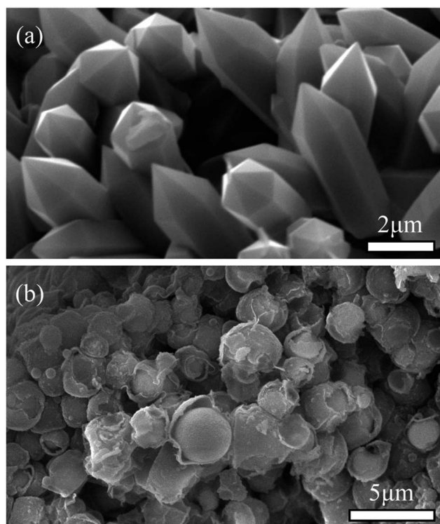
Fig. 32 SEM images of thermal decomposition residue of [\text{ZnCl}_2\text{L}] (a) and [\text{ZnBr}_2\text{L}] (b) calcined at 500^\circ\text{C} for 2 h. [Reproduced from ref. 320 with permission from The Royal Society of Chemistry.]
