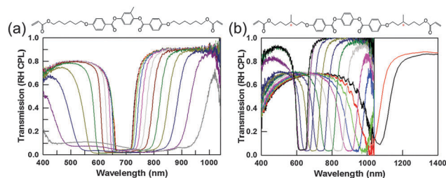
Fig. 1 Electro-optic response of PSCLCs prepared with 5 wt% polymer concentration: (a) bandwidth broadening observed in a formulation (b-PSCLC) prepared with RM82 (inset) at 0–110 V DC and (b) red notch tuning at 0–100 V DC in a formulation (t-PSCLC) prepared with SLO4151 (inset). The probe of the light source used to collect the transmission spectra was right handed circularly polarized to match the handedness of the PSCLC samples.
