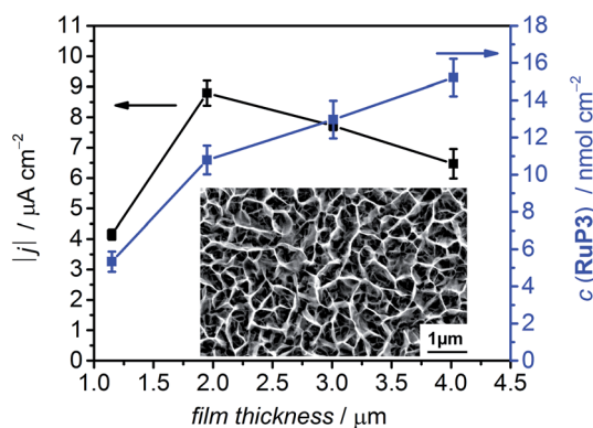
Fig. 3 Photocurrent response of NiO| RuP3 under visible light irradiation ( \lambda > 400 nm, AM1.5G filter, 100 mW cm^{-2} ) after 100 s at E_{appl} = 0.3 V vs. RHE in Na_2SO_4 (0.1 M, pH 3) in the presence of 4,4'-dithiodipyridine (DTDP, 1 mM) as SEA and dye loading (no applied potential; cm^{-2} refers to the geometrical surface area of the NiO electrode) with varying thicknesses of the NiO films. Inset: SEM image of optimised p-type NiO electrode (2 \mu m film thickness).
