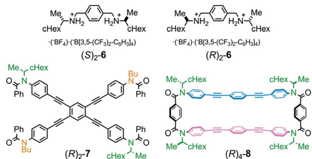
Fig. 2 Chemical structures of chiral ditopic guests (S)_2-6 /( R ) _2-6 , and references (R)_2-7 and (R)_4-8 .
